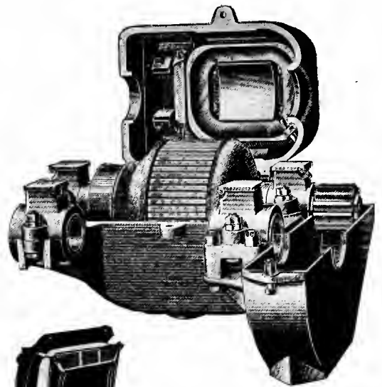
Fig. 5675. MOTOR-CASE AND ATTACHMENT TO AXLE.
